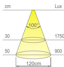
* values referring to FLEXYLED HE8B 1000mm 4000 K
